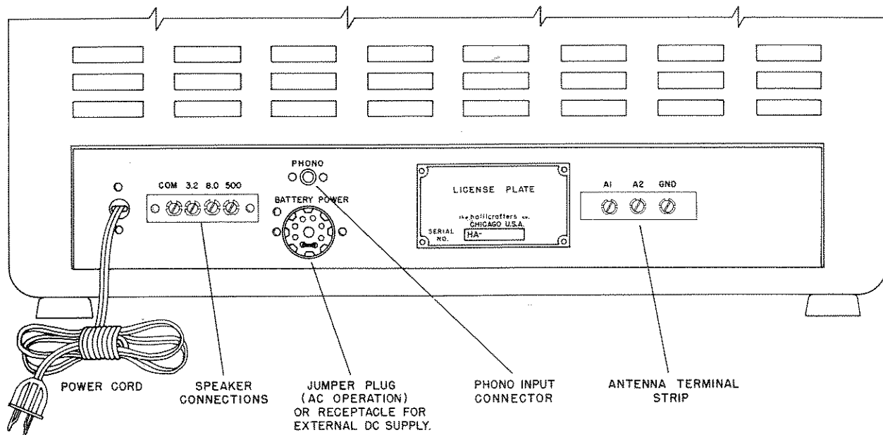
Fig. 3. Rear view.
