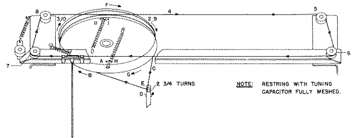
Fig. 7. Dial cable stringing procedure
