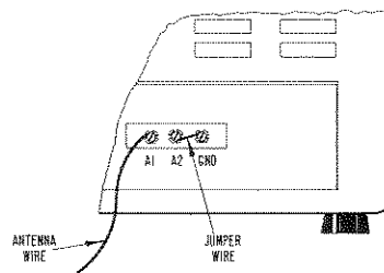
Fig. 4. Single Wire Antenna
