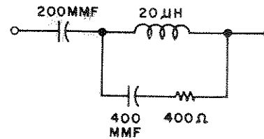
Fig. 4. RETMA Dummy Antenna
